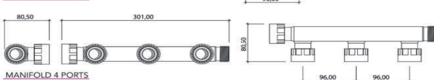
MANIFOLD 4 PORTS
