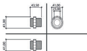
NIPPLE 1"
