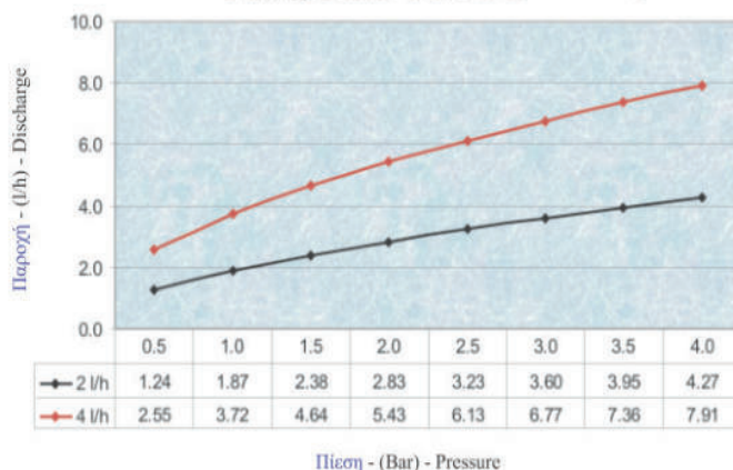
Paladrip 16mm - 2 & 4 LPH
