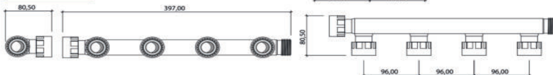
MANIFOLD 4 PORTS
