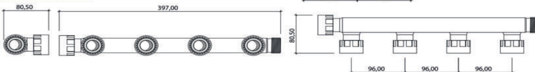
MANIFOLD 4 PORTS
