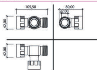
TEE FxFxM 1"
